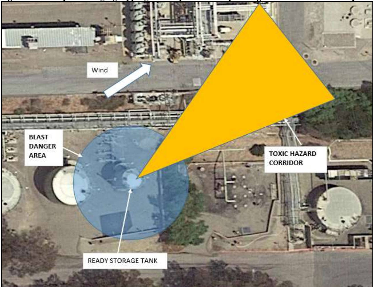
Figure 1 - Example: Charging Hypergolic Propellant Ready Storage Tank at Launch Complex
